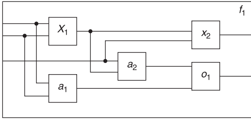
Figure 26.8 A circuit diagram of the full adder described in text box, after © 1987 Morgan Kaufmann publishers.
