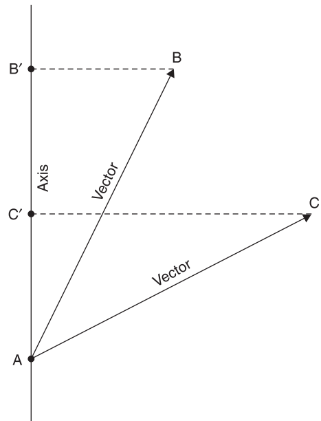
Figure 3.5 Computing the amount of information in a vector explained by an axis. Draw a line from the tip of the vector to the axis, perpendicular to the axis. The amount of information resolved by the axis is the ratio of the projected length on the axis to the true length of the vector. If a vector lies close to the axis, then this ratio is high and most of the information in the vector is resolved by the axis. Vector AB lies close to the axis and the ratio of the projection AB' to the vector itself, AB , is high. Vector AC lies far from the axis and the ratio of its projected length AC' to the vector itself, AC , is low.
