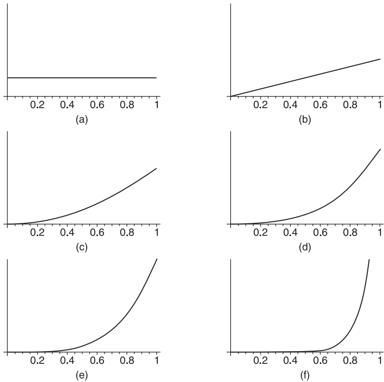
Figure 17.3 The change in my subjective probability density as more and more black ravens are observed.
