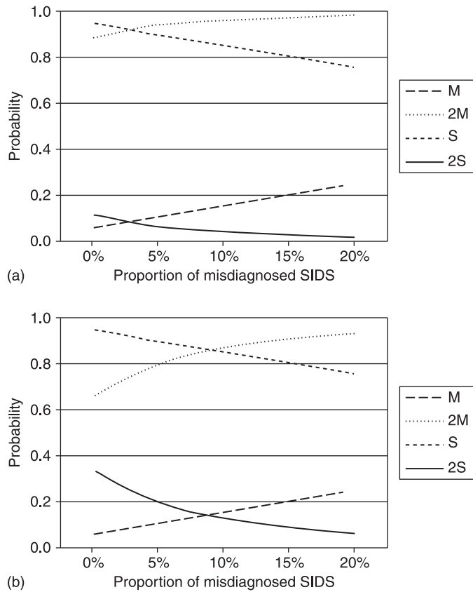
Figure 30.1 (a) Prior probabilities of SIDS and murder (SIDS independence). (b) Prior probabilities of SIDS and murder (SIDS dependence).
