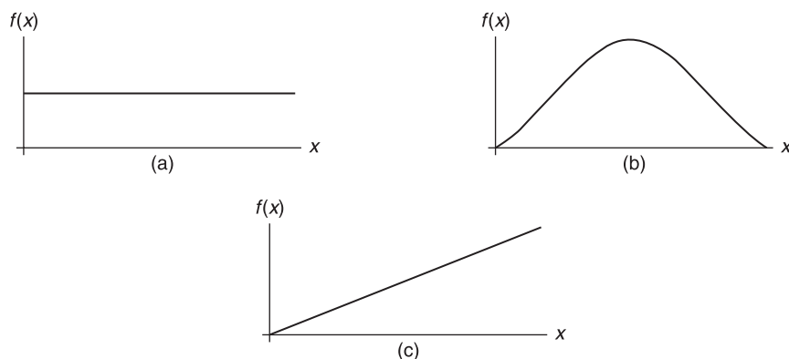
Figure 17.2 Some choices of prior probability density for the raven blackness hypotheses.
