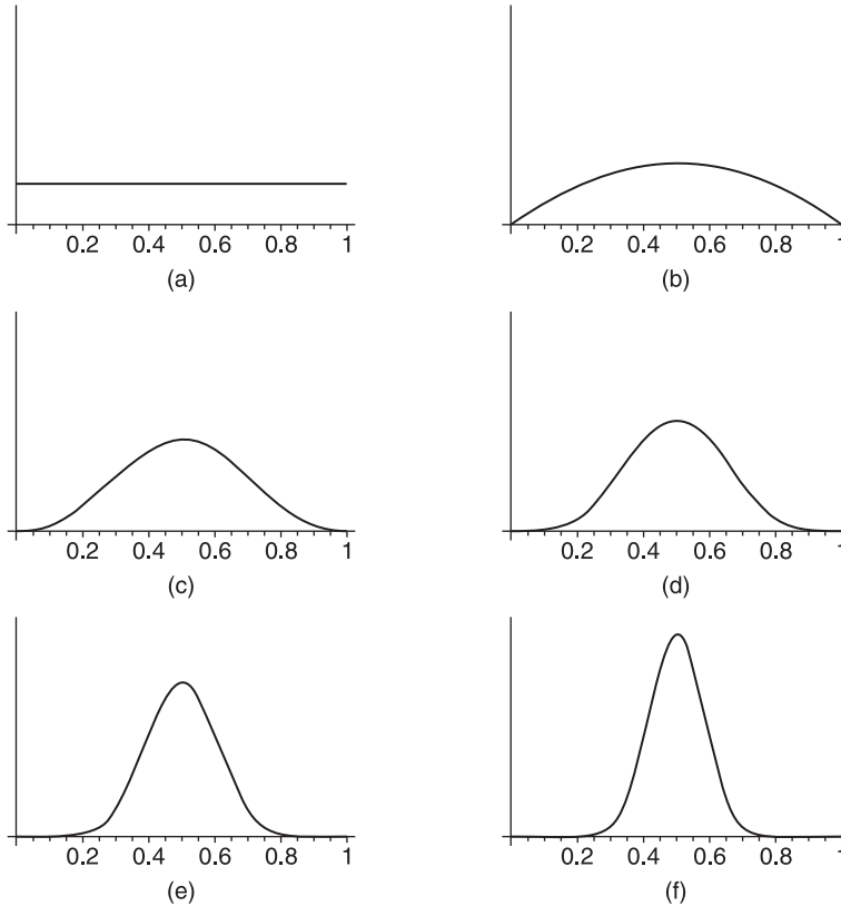
Figure 17.4 The change in my subjective probability density as more and more ravens are observed, if half of all observed ravens at any stage are black.
