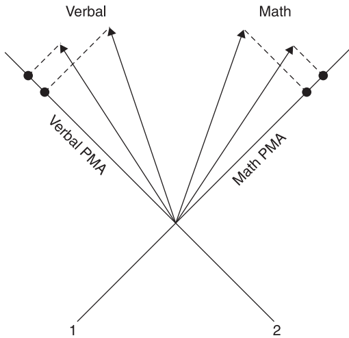
Figure 3.7 Rotated factor axes for the same four mental tests depicted in Fig. 3.6. Axes are now placed near vectors lying at the periphery of the cluster. The group factors for verbal and mathematical aptitude are now well identified (see high projections on the axes indicated by dots), but g has disappeared.
