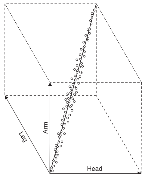
Figure 3.3 A three-dimensional graph showing the correlations for three measurements.
