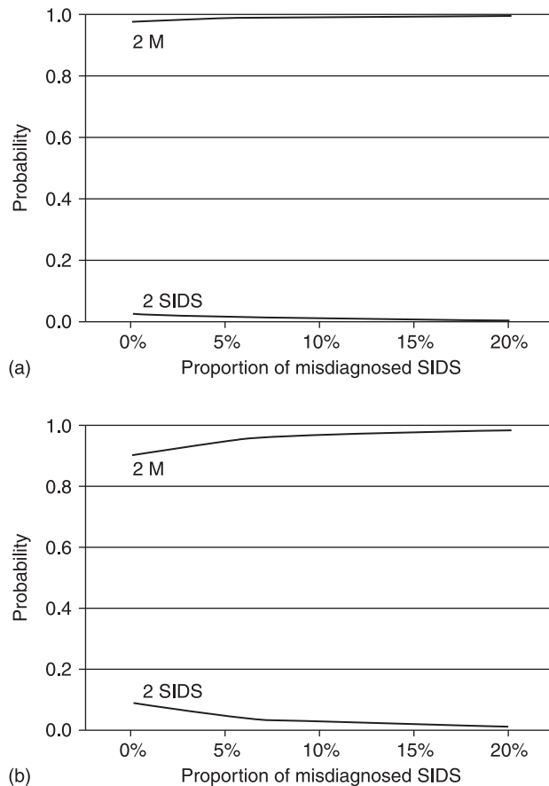
Figure 30.2 (a) Posterior probabilities of double SIDS and double murder (SIDS independence), (b) Posterior probabilities of double SIDS and double murder (SIDS dependence).
