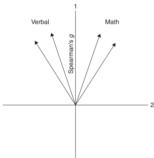
Figure 3.6 A principal components analysis of four mental tests. All correlations are high and the first principal component, Spearman's g , expresses the overall correlation. But the group factors for verbal and mathematical aptitude are not well resolved in this style of analysis.
