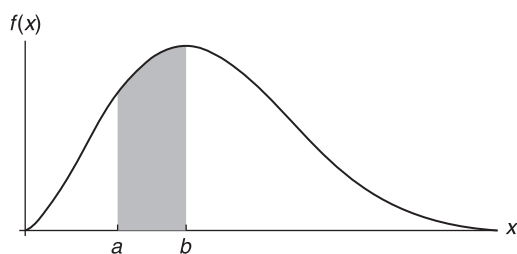
Figure 17.1 A probability density over the raven hypotheses.
