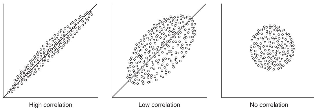
Figure 3.1 Strength of correlation as a function of the shape of an ellipse of points. The more elongate the ellipse, the higher the correlation.
