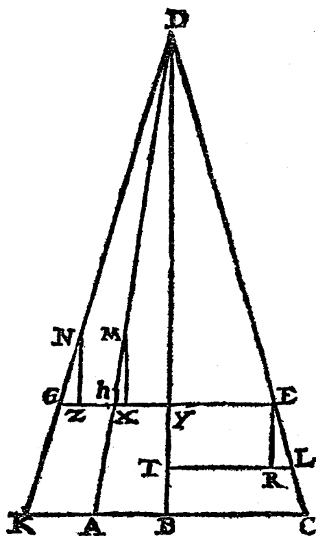
Figure 1.7. Inclined plane according to Tartaglia ( Quesiti ). According to Tartaglia, two weights at E and H along planes with the same height DB , but of different inclinations DC and DA , have the same powers to descend if the weights are proportional to the lengths of their respective planes. Tartaglia's diagram tries to explain the inclined plane by means of another plane DK with a slope equal to that of DC . Tartaglia makes no attempt to account for the inclined plane in terms of the lever; rather, he uses the notion that bodies have a greater tendency to descend the closer their descent is to the vertical.
