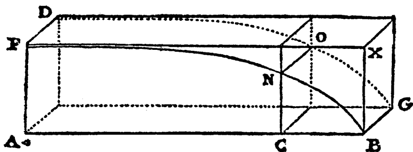
Figure 3.15. Parabolic beam ( Discorsi ). The beam ABGDF with a parabolic profile, infixed in the wall at AFD and loaded at BG , offers the same resistance at any point C along its axis. In the parabola, BA is to BC as AF^2 is to NC^2 , but the resistance of each cross-section is as NC^2/BC , which is constant, therefore the resistance is constant at any point C along the axis.
