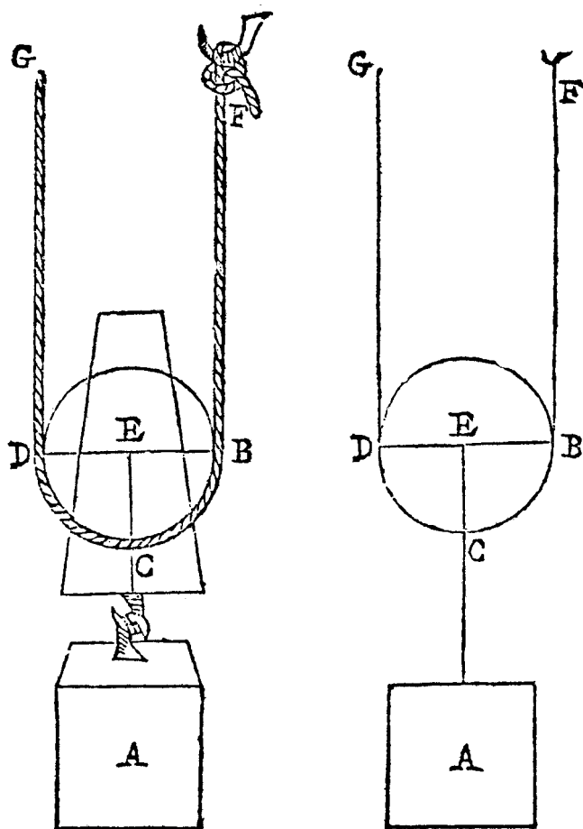
Figure 1.5. Dal Monte's pulley and balance ( Mechanicorum liber ). Once again, as in figure 1.2, dal Monte depicts both a real machine and a geometrical one. DEB is, as it were, a lever with the fulcrum in B and the weight appended in E . The power is applied in D (or G ). In this case, if we assume the pulley itself to be weightless, the power is half the weight of the body A because the arm BD is twice the arm BE . More elaborate arrangements with more pulleys can reduce the power and resistance further.
