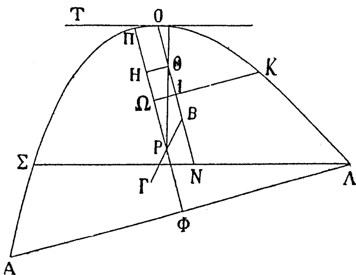
Figure 2.2. A proposition from Archimedes' Floating Bodies , book 2. The figure is obtained by rotating a parabolic sector around its axis. The equilibrium conditions depend on the positions of the centers of gravity of the whole body and of the part immersed in the fluid, where ΣΛ is the surface of the fluid.
