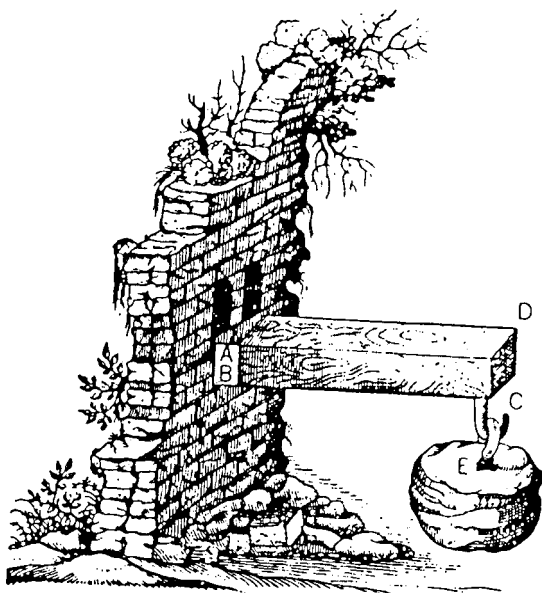
Figure 3.13. Galileo's beam ( Discorsi ). Galileo tried to determine the resistance of a beam ABCD infixed at right angles in a wall, or cantilever, by means of the lever. B is its fulcrum, BC is one of its arms, and BA is the other at right angles to it. The moment of the weight E in C is counterbalanced by the moment of the beam's resistance to breaking, proportional to the number of fibers in its base or to the area of the cross-section. Since the fibers are equally spaced, they work as if they were all in the middle point of AB , by analogy with a system of weights. Thus the resistance to breaking is as the cross-section times half the height.
