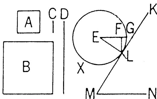
Figure 1.6. Inclined plane according to Pappus ( Collections ). According to Pappus, a given force C is required to move a weight A over a horizontal plane. It is required to find the force needed to move a sphere of weight A up on an inclined plane MK . The key idea consists in imagining a balance EG , parallel to the horizon, where the fulcrum F is on the perpendicular from the point of contact L of the sphere and the inclined plane. The weight A of the sphere acts on its center E , and the force D is required to keep the weight B in equilibrium by pulling down on G . This reasoning relies on the assumption that the sphere rolls without sliding. Weight B is to weight A as EF is to FG , which can be determined by elementary geometry. Therefore we also have force D . This force tends to become infinite as the inclined plane tends toward the vertical. The force required to move the sphere up on the inclined plane is C plus D , namely the force required to move it along the horizontal plus that required to keep it in equilibrium balancing its weight. Pappus included in his figure two squares representing weights A and B , and two lines representing forces C and D , so as to give geometrical representation to all the magnitudes he discusses.
