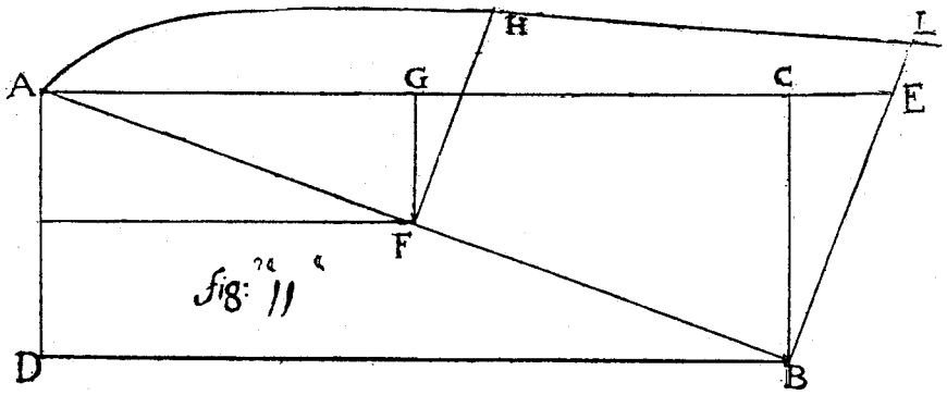
Figure 6.7. Guglielmini's law of efflux ( Aquarum fluentium mensura ). According to Guglielmini, the law of efflux rules water flow and determines also the speed of the water of a river. At F , for example, the speed is proportional to the square root of the segment FG , representing the distance to the horizontal AE from the source A .
