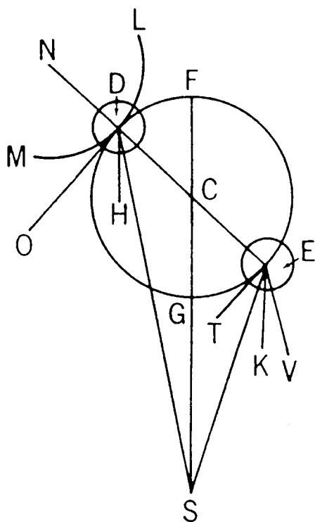
Figure 1.4. Dal Monte's lines of descent ( Mechanicorum liber ). In this complex diagram DCE represents the tipping balance with weights in D and E . Angles KET and HDO are equal. According to Tartaglia, the body in D would be heavier than the body in E because the angle HDG would be smaller than the angle KEG . The difference would come from the angles of contact TEG (between the tangent TE and the arc EG ), which has to be added to KET , and ODG (between the tangent DO and the arc DG ), which has to be subtracted from HDO . According to dal Monte's hypothetical reasoning, angle SEG would be smaller than SDG , where S is the center of the Earth; therefore the body in E would be heavier. Thus, rather than returning to the horizontal position, the balance would move downward. On the mistaken interpretation by Duhem and his followers, this diagram would be the hallmark of dal Monte's pedantry because of his belief that the lines of descent of the weight of a balance are not parallel among themselves but converge toward S .
