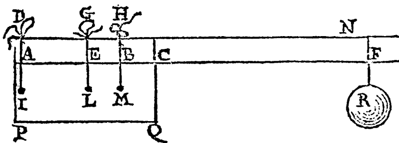
Figure 8.14. Mariotte's balance ( Traité du mouvement des eaux ). A balance AEBCF is secured with three strings ID , GL , and HM to a block PQ , and a weight R is attached at F . C is the fulcrum, and CF = 12 feet, CA = 4 feet, CE = 2 feet, and CB = 1 foot. The strings break when they are stretched two lines. Taking them one by one, because of their respective distances, DI breaks if R = 4 pounds, GL breaks if R = 2 pounds, and HM breaks if R = 1 pound. If we take them together, however, HM can stretch only one-quarter of its maximum extension and LG only one-half, otherwise DI would break. Since the degree of stretching is proportional to the strings' load, HM supports only \frac{1}{4} pound and GL only 1. Generalizing, the load each string supports varies as the square of the distance from C . A similar reasoning can be applied to a beam infixed in a wall, namely Galileo's case. After an extraordinarily contorted calculation, corresponding in the language of calculus to the integration \int x^2 dx , where x is the distance from the fulcrum, Mariotte was able to show that the coefficient he was seeking was not \frac{1}{2} , as Galileo had thought, but \frac{1}{3} .
