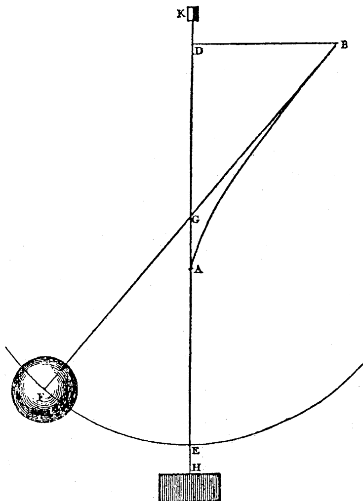
Figure 7.12. Huygens's isochronous conical pendulum ( Horologium oscillatorium ). The pendulum consists of a thread BGF , with a weight in F , rotating parallel to the horizon around the axis DH . The thread rests on the curved plate BA , and the faster it turns, the higher it rises. The plate BA is shaped like a paraboloid whose evolution describes the parabola EF . This condition makes the pendulum's rotation isochronous, much like cycloidal motion for the vertical pendulum.
