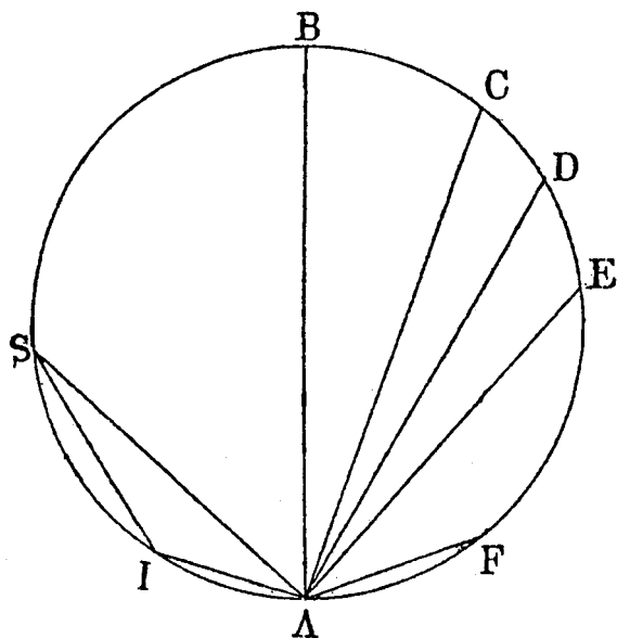
Figure 3.2. Galileo's chord theorem (1602 letter to dal Monte). A body falls in equal times along the diameter BA of a circle and along its chords CA , DA , EA , and FA . One of Galileo's attempted proofs relies on the idea that the speeds are as the momenti . If the momenti are as the distances, the speeds are as the distances as well, and the motions occur in equal times. Paradoxically, the proof may also be applied to uniform motions.
