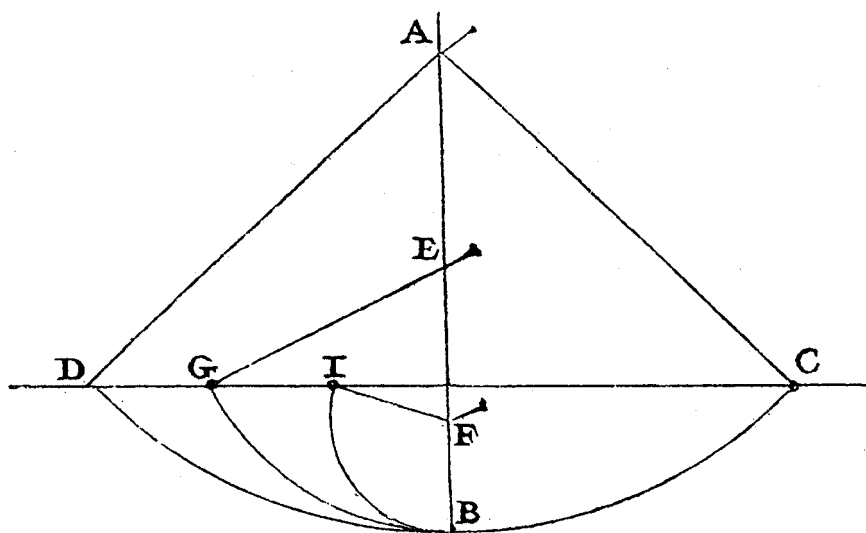
Figure 3.16. Galileo's pendulum ( Discorsi ). Galileo's esperienza consists in inserting a nail at different heights such as E and F on the vertical of an oscillating pendulum. The bob will always reach the same height D , G , or I along smaller arcs, and from there it will reach back up to C . Hence it has the same speed in B as long as it falls from any point on the line CD . Here Galileo considered a circle arc as an infinite series of inclined planes with different inclinations.
