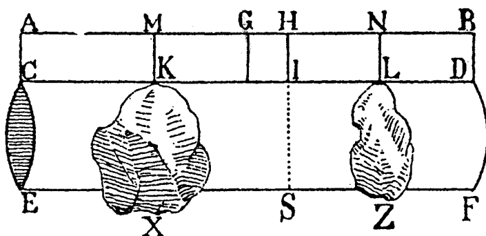
Figure 3.1. Galileo on the equilibrium of the balance ( Le mecaniche ). A solid of uniform density CDFE is attached by the extremes C and D to a balance AB suspended from its middle point G . If we cut it along IS and suspend both parts from the balance by string IH , the system will still be in equilibrium. If we now suspend the two unequal parts by their middle points K and L , by means of KM and LN , and cut strings AC , HI , and BD , the two solids will remain in equilibrium. Now the two weights CS and SD , or KX and LZ , must be of equal moment. Galileo can show that NG:GM::CS:SD . Therefore the balance is in equilibrium if the weights are inversely as the distances from the fulcrum at which they are hung.
