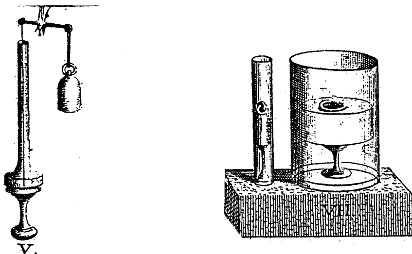
Figure 6.4. Pascal's hydraulic paradox ( Physical Treatises ). In figure V Pascal used the balance to highlight a hydraulic paradox, whereby a large weight holding the bottom of the tube in place by means of a thread is needed to counterbalance a tiny amount of water in the narrow tube. In figure VII a small weight keeps a large one in equilibrium through the hydraulic press.
