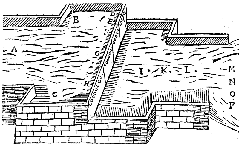
Figure 6.2. Castelli's thought experiment ( Della misura ). Castelli's thought experiment intended to show that the quantity of water flowing in a canal is as the square of the water's height.
