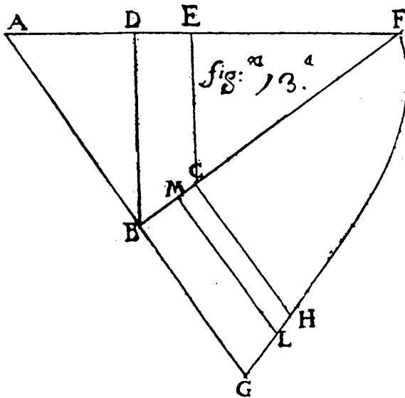
Figure 6.8. Guglielmini's profile of speeds in a river ( Aquarum fluentium mensura ). The profile of speeds FHLG along river AB resembles that in figure 6.6, which appears rotated by about 45 degrees. Notice that the surface speed at F is nil, because AF is the parallel to the horizon from the source A .
