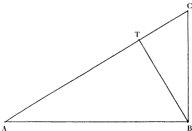
Figure 3.10. Galileo's inclined plane ( Dialogo ). Given the inclined plane ABC , Galileo could prove that in the time it takes a body to fall along the vertical CB , another body released at the same time and falling along the incline will reach point T . This result derives from the assertion that the time of fall along the inclined plane CA is to the time of fall along the vertical CB as CA is to CB . Since the times are as the lengths, applying a well-known theorem by Euclid we have CA:CB::CB:CT . Galileo's claims are sound for sliding bodies, but if rolling is involved they become problematic, as Mersenne was to show. See chapter 4.
