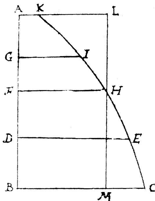
Figure 6.6. Guglielmini's profile of speeds in a river ( Aquarum fluentium mensura ). The river is of depth AB , and AK , GI , FH , etc., are the speeds at corresponding heights A (the surface), G , D , etc. FH is the average speed. This illustration should be considered together with the following two, which explain why the profile of speeds is parabolic and how the surface speed AK is determined.
