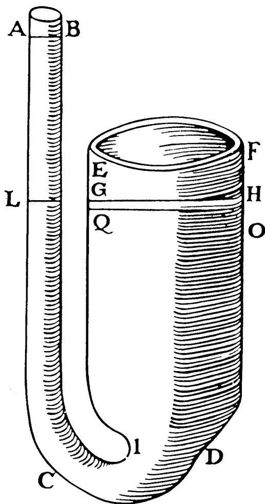
Figure 3.8. Galileo's siphon (1612 Discorso ). Water in the two containers EIDF and ICAB is in equilibrium if it is at the same level, regardless of their cross-sections. According to Galileo, the system works like a balance wherein a small motion of the water in the large container, to QO for example, makes the water in the thin container rise in the same time from L to AB . The speeds are inversely as the cross-sections, but since the cross-sections are as the weights in GD and LC , the speeds are inversely as the weights, just as in the balance. Therefore the different speeds compensate for the different weights, and the moments are equal.
