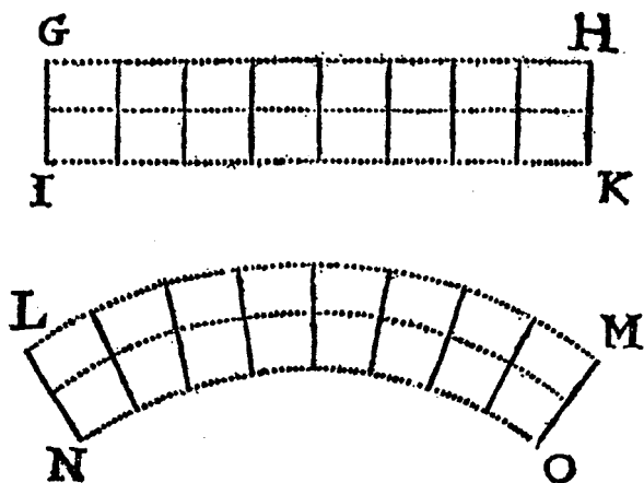
Figure 8.9. Hooke on compound bending ( De potentia restitutiva ). The picture shows a straight solid body GHKI and then the same body bent LMON . The side LM is extended, while NO is compressed.
