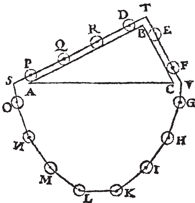
Figure 1.8. Stevin's inclined plane ( Elements of the Art of Weighing ). In the case studied by Stevin, in the triangle ABC the side AB is twice BC , and the wreath has fourteen spheres overall, four on AB and two on BC . This conclusion can be easily generalized to the case where one of the planes is vertical. Since the lower part can be removed by symmetry considerations without altering the equilibrium conditions, the two portions at the top must be in equilibrium; hence weights have to be proportional to the length of the inclined planes.
