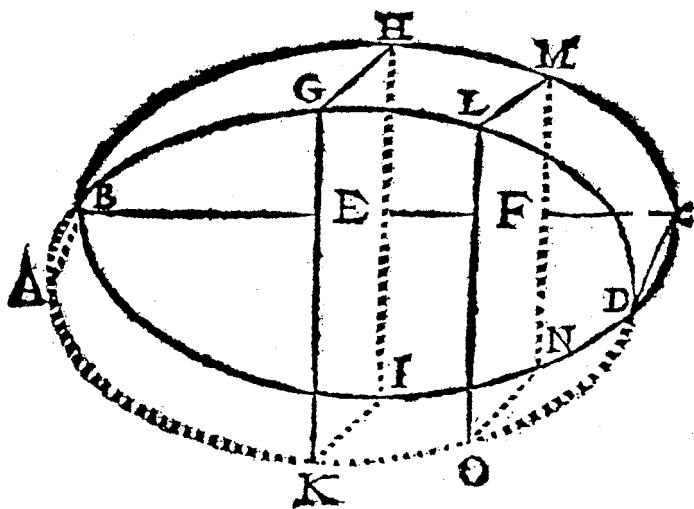
Figure 8.11. Marchetti on the resistance of materials ( De resistentia solidorum ). ABCD is a solid body with an elliptical profile. Marchetti's proposition argues that the resistance in E is to the resistance in F as FB \times FC \times HI^2 is to BE \times CE \times MN^2 . Since in an ellipse HI^2 is as BE \times CE and MN^2 as FB \times FC , it follows that the ratio between the two resistances is the unity. Therefore a beam with an elliptical, or circular, profile offers at any point the same resistance to a given load.
