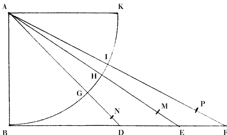
Figure 8.7. Fabri's attempt to prove isochronism ( Physica ). In the quadrant ABGHK the radius AB represents the length of the cord not subjected to tension. The cord can be taut from G to D , from H to E , or from I to F , for example, which are as 1, 2, 3. Fabri claimed that if in a given time D moves to N , in the same time E will move to M such that EM = 2DN . He justified this claim by arguing that motion is proportional to the displacement, and therefore the motions along EM and DN are as EM and DN themselves. Fabri divided GD into four equal parts, the first one being DN , arguing that once released, the string will move through DN in the first instant and through NG = 3DN in the second. Likewise, in the same time E will move first to M and then to H , where HM = 3ME . The same applies to AIF , for symmetry reasons. Fabri sought to prove his proposition with proportions and finite, rather than infinitesimal, time intervals. He was aware that he was applying Galileo's odd-number rule to a case in which acceleration is not constant, but he argued that regardless of how acceleration increases, motion is always proportional to the displacement, and therefore oscillations are isochronous.
