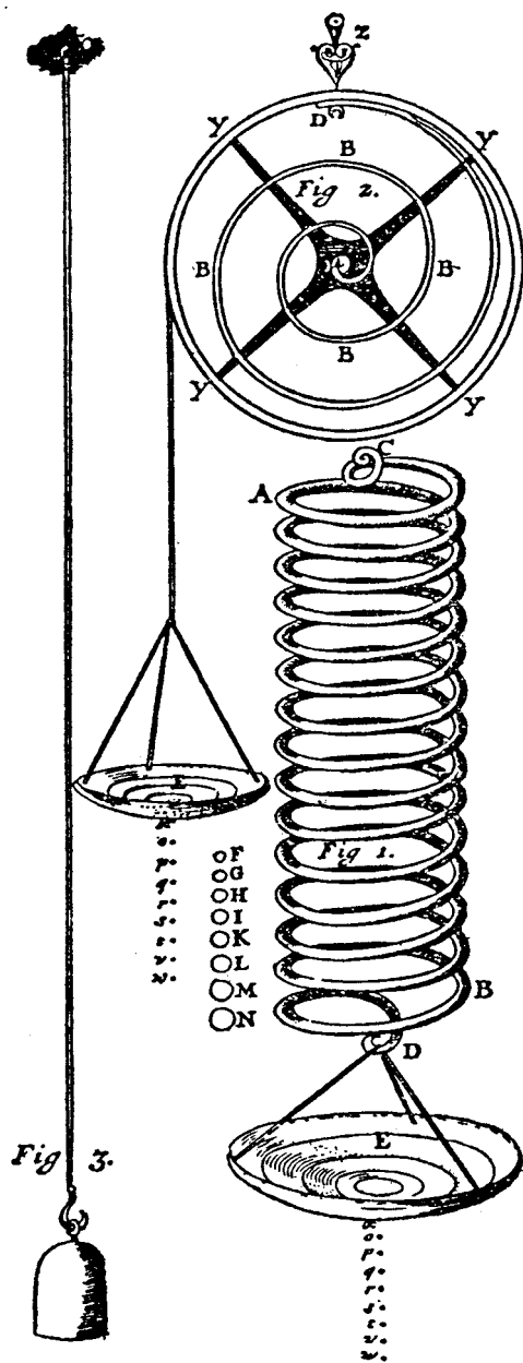
Figure 8.8. Hooke's springs ( De potentia restitutiva ). Hooke's experiments with different types of springs showed that the displacement is as the power, or force, applied.
