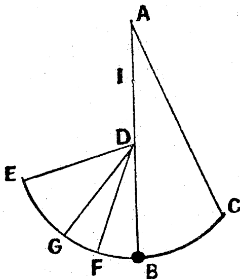
Figure 7.3. Borelli's pendulum ( Theoricæ Mediceorum planetarum ). Borelli claimed that the speed of a body moving along the arcs BC or BE is the same, although the angular distance covered in the same time is greater over BE than BC . He tried to prove this statement by arguing that the speed of a bob would be the same whether AB is free or hindered by a nail in D . The idea of using a nail in D to shorten the pendulum is clearly borrowed from the third day of the Discorsi (fig. 3.16). Borelli claimed that the bob would reach point G . Surprisingly, he did not state that C and G should be at the same height, but rather claimed on the basis of experience that the angles G\hat{D}B and B\hat{A}C are inversely as the square roots of the lengths of the pendulums, \sqrt{AB}:\sqrt{DB} . From here Borelli argued that the speeds of the pendulum are equal and also that without external influences, the speed of an orbiting body would be constant and the body would traverse equal distances in equal times at different distances from the center. The analogy between the vertical pendulum and an orbiting body is problematic, however, because an orbiting body at a constant distance from the center has a constant speed, whereas the speed of the pendulum varies at each point.
