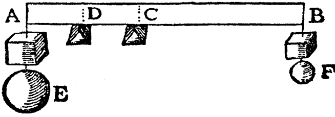
Figure 3.14. A beam supported at both ends ( Discorsi ). In order to study a beam supported at both ends and loaded with a weight at some point on its axis, Galileo considered the case of a beam supported at some point on its axis and loaded at both ends. He argued that the smallest forces A, B required to break the beam in C are to the smallest forces E, F required to break the beam in D as AD \times DB is to AC \times CB .
