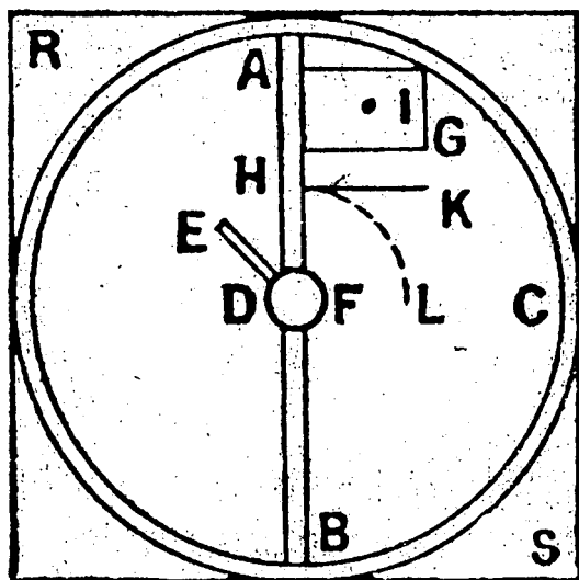
Figure 7.2. Borelli's bowl ( Theoricæ Mediceorum planetarum ). A wooden circle ABC with a wooden diameter AB is in a container full of water RS . A magnet F is in the center D . I is an iron ball floating on a small piece of cork G capable of moving freely on the water. When one moves the cork with the ball sufficiently close to the magnet F , the ball starts being attracted. If at this point one rotates the whole wooden frame ABC , the diameter pushes the ball and makes it rotate. If the magnetic attraction is compensated by the tendency HK generated by the circular motion to move away from the center along the tangent, then the ball I will be in equilibrium, just like a planet with respect to the sun or a satellite with respect to a planet. In his typical style, Borelli also provided an alternative account without the magnet and the floating cork. This time the diameter AB is not flat but raised in A and B , so that a ball placed on it tends to slide toward D along a groove cut in AB . By rotating AB , so as to have two rotating inclined planes, it is possible to generate a force opposed to the weight of the ball so that the ball stays in equilibrium. In some respects his approach is not entirely dissimilar to Huygens's, as we shall see below.
