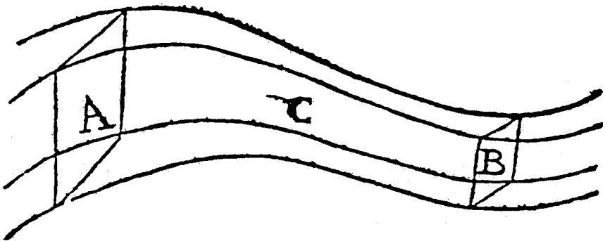
Figure 3.9. Proposition 1 from Castelli's Della misura . Castelli showed that the quantity of water flowing through sections A and B of a river in a steady state must be the same, and that water cannot be compressed; therefore the speeds at A and B are inversely as the respective cross-sections. Although Galileo studied pipes and Castelli rivers, Castelli's figure looks like a straightened version of Galileo's siphon shown in figure 3.8.
