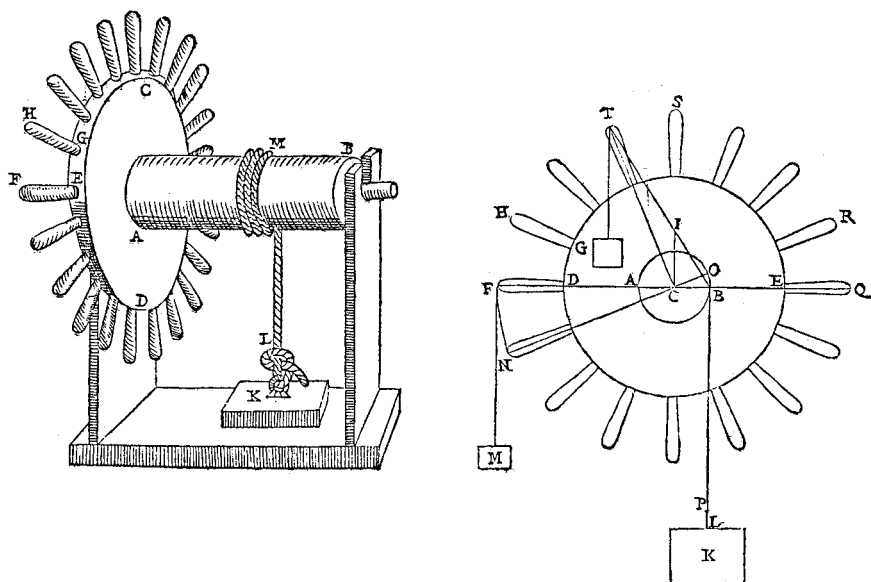
Figure 1.2. Dal Monte's wheel and axle ( Mechanicorum liber ). A rope is wrapped around the cylinder AB so that by turning the handles H, F, N , etc., weight K is raised. The force on the handles is represented by the attached weights G or M . Here dal Monte identifies the arms of the lever as the radii CF and CB , C being the fulcrum. By pushing on F, N , etc., we can raise the weight K with a smaller weight M , albeit more slowly than by pulling it directly. The lever as seen by dal Monte has disjointed arms: CB is always parallel to the horizon, whereas CF may rotate around C . Notice that weight M is perpendicular to the arm FC , whereas in all other positions such as TC or NC we have to take into account only the component perpendicular to the arm, which changes with the angle of inclination; therefore, as dal Monte states, weight G attached in T is greater than weight M . The illustration reproduced in Mechanics in Italy , 318, is inaccurate in that G is not drawn larger than M .
