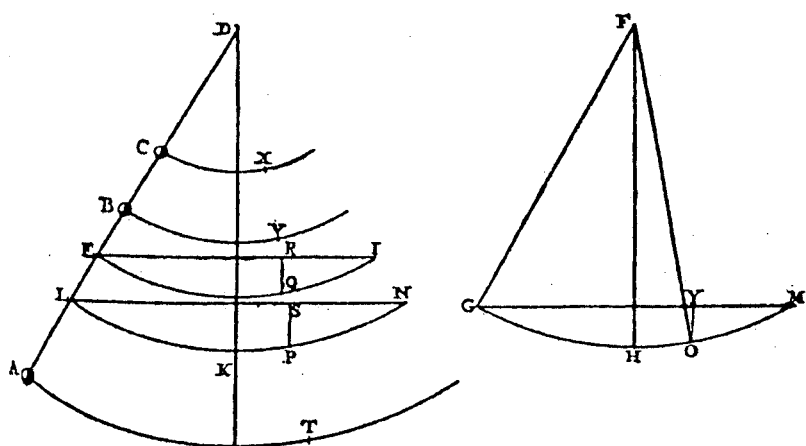
Figure 7.9. Huygens's compound pendulum: the formal presentation ( Horologium oscillatorium ).
