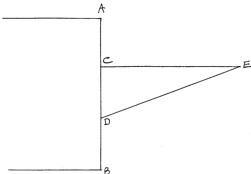
Figure 8.12. Fabri's prism (adapted from Physica ). CDE is a prism infixed in a wall AB seen from the top with a triangular base. Fabri's prism is a solid of equal resistance and is both simpler and lighter than Galileo's parabolic beam. By keeping a constant height, Fabri had simple as opposed to quadratic proportions among variables, notably between width and length.
