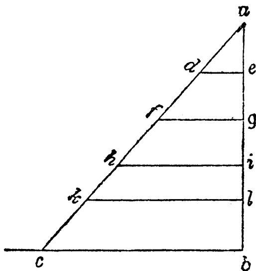
Figure 3.4. Inclined plane and triangle of speeds (elaboration of Galileo's manuscript 179v). For an object falling from a along the vertical ab or an inclined plane ac , the speed of fall is the same at the same vertical distances ed , gf , etc., from the vertex a . If the vertical represents a distance, we have a spatial representation of fall along an inclined plane, but if it represents time, we have a graph known as the triangle of speeds where ed , gf , etc., represent increasing speeds at different times, each known as gradus velocitatis . At times Galileo mixed the two, claiming that speeds are as the distances. If ab represents time, cb represents the maximum degree of speed. The mean-speed theorem states the equality of the distances traversed in equal times with a uniformly accelerated motion from rest, or with a uniform speed equal to the mean degree of speed of the accelerated motion. Galileo replaced the mean degree of speed with half the maximum speed cb (see also fig. 3.17). The double-distance rule states that the distance traversed with a uniform speed equal to the maximum degree of speed cb acquired with a uniformly accelerated motion from rest is double the distance traversed with that accelerated motion in the same time.
