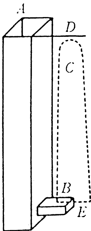
Figure 4.8. Torricelli's pierced cistern ( De motu ). In tackling the problem of the pierced cistern, Torricelli identified features analogous to the equilibrium of water in conjoined containers and to the motion of projectiles. He arranged for the jet of water spurting out at B to be projected upward and showed that it almost reached the level AD of the water in the tank. Since in falling to E after having reached its maximum height C the jet goes through the same degrees of speed as in rising, at E the water must have the same speed it had at B when coming out of the orifice; hence the water can be imagined as falling inside the container almost as if it were a body falling in air, and its speed at B is as the square root of the height of the water in the container.
