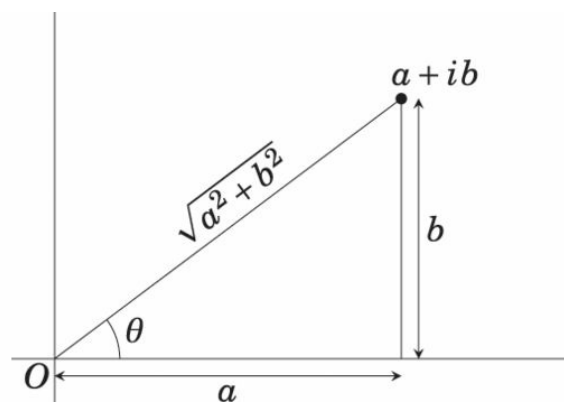
Figure 10 The geometry of a complex number.
