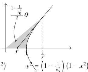
Fig. 4.3 Paraphrase of the steps Newton used to derive his description of trajectories in an inverse-cube force field
