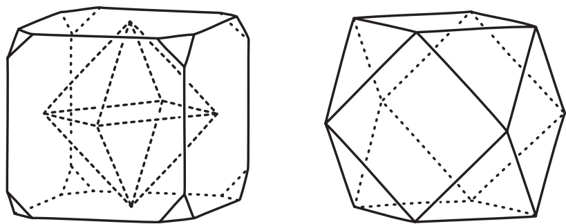
Figure 1.2. Cleaving fluorspar. 5
