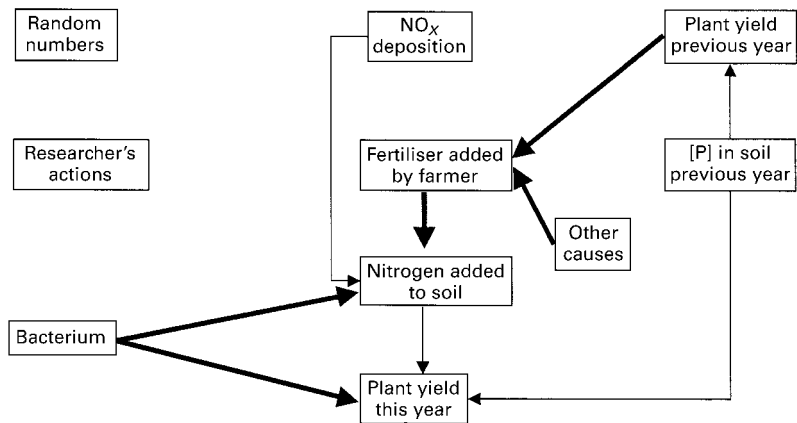
Figure 2.16. A hypothetical causal system before experimental manipulation.
