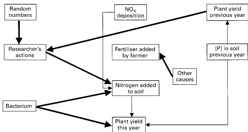
Figure 2.18. Experimental manipulation of the causal system shown in Figure 2.16 that is not based on a randomised experiment.
