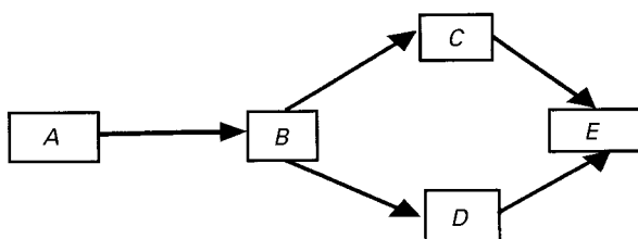
True causal graph
