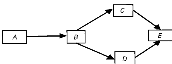
True causal graph
