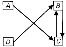
Figure 8.37. The partially oriented ancestral graph that results from the Cyclic Causal Discovery algorithm is shown on the left followed by the two equivalent cyclic graphs.
