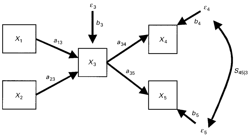
Figure 4.1. A path model involving five variables; S_{45|3} is a free covariance between \varepsilon_4 and \varepsilon_5 .
