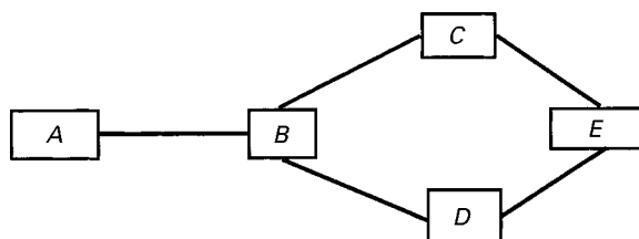
Figure 8.8. The true (unknown) causal graph and the resulting undirected dependency graph.
