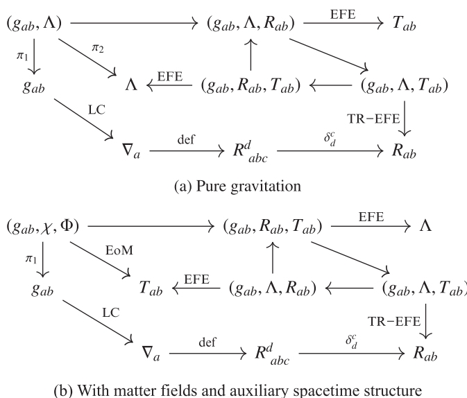
Figure 1 Commutative diagrams of the determination relations for models of GR, in the “pure” case and the case with matter and auxiliary spacetime structure. Among the objects, g_{ab} is the metric, \Lambda is the cosmological constant, \chi is the auxiliary spacetime structure, \Phi is the collection of matter fields, \nabla_a is the affine connection, T_{ab} is the energy–momentum tensor, R^d_{abc} is the Riemann tensor, and R_{ab} is the Ricci tensor. Among the arrows, \pi_i is the i th component projection, \delta is the delta (contraction) tensor, “def” is a mathematical definition, “EoM” is the assignment of energy and momentum from the matter fields, “EFE” is the Einstein field equation, and “LC” is the Levi-Civita construction. All arrows not labeled follow from the universal property of products. (Note that the trace-reversed arrows are not needed for these.) Inessential identity and projection arrows are omitted.
